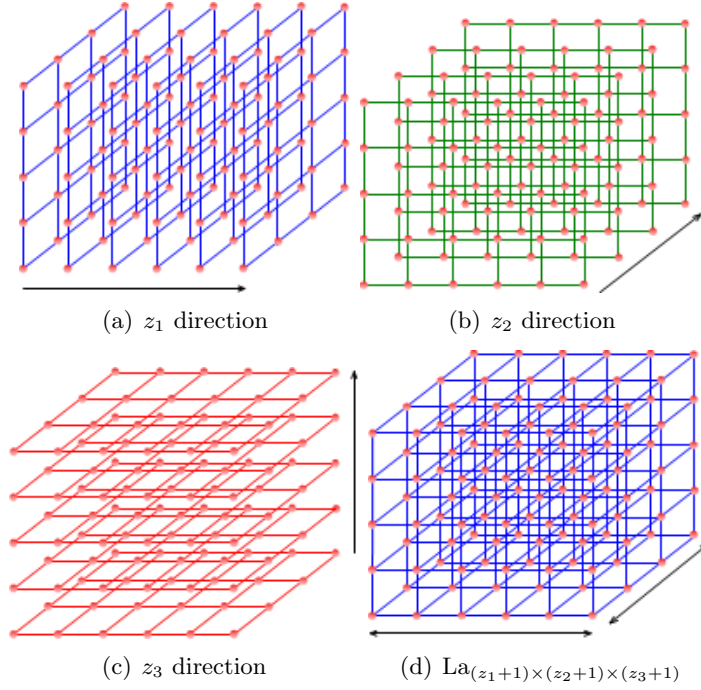
Figure 2: Construction of 3-dimensional lattice
