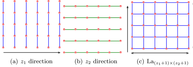
Figure 1: Construction of 2-dimensional lattice
