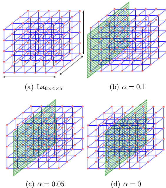
Figure 4: Partitioning of three-dimensional lattice \text{La}_{6 \times 4 \times 5}
